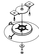
Magnetic/Suction Mount
