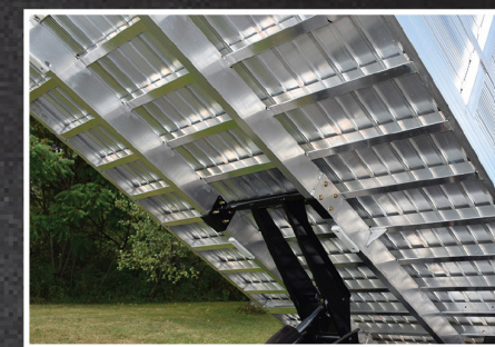
Standard HD Subframe with 12" OC Cross Members
